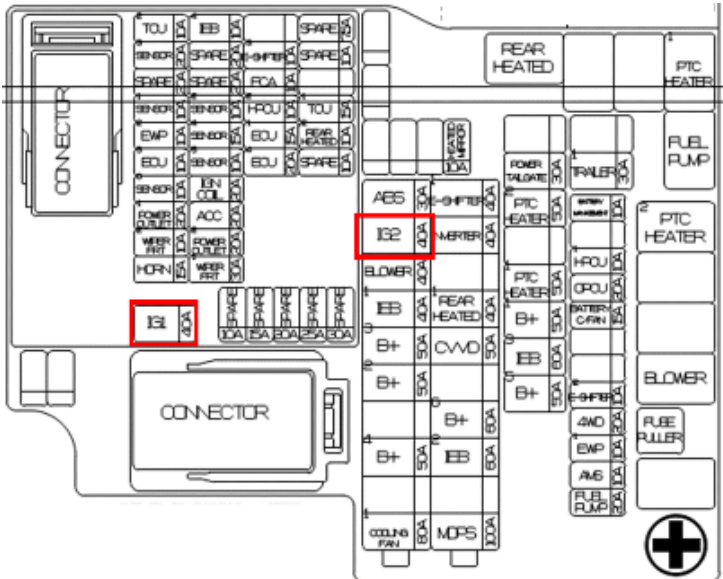
Engine room fuse box
